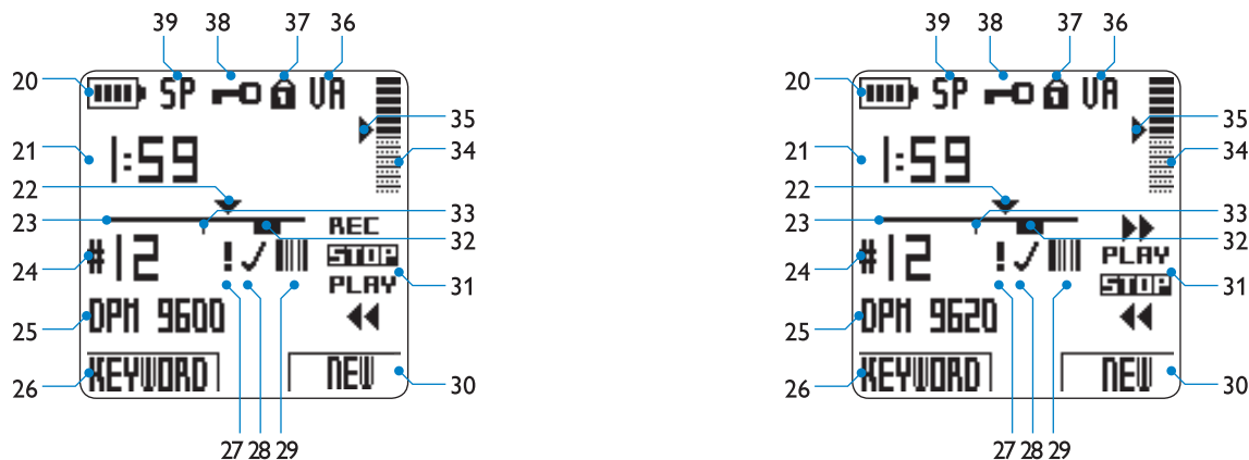
Digital Pocket Memo 9600
