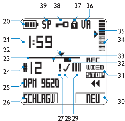
Digital Pocket Memo 9600
